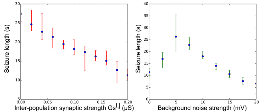
Fig 8. Seizure lengths according to inter-population coupling (left) and background noise (right). Simulations were performed to reproduce 15 minutes of activity for each parameter setting, resulting in 10 to 30 seizures per simulations. Mean, minimum and maximum seizure lengths were calculated from these generated time series by isolating the fast firing neurons' activity and counting the time spent in up-state (threshold at -40 mV). Up-states of less than 5s were not considered as seizure and down-states of less than 3s between consecutive seizures were considered as being part of the same seizure. Noise is inserted in both excitatory and inhibitory neurons. Parameters: C_E = 0.8 , x_0 = 3.0 ; W_{max} = 0.2 (left plot); G_s^{ij} = 0.1 (right plot); G_s^{ij} = 0.1 ; r = 0.000004 .
