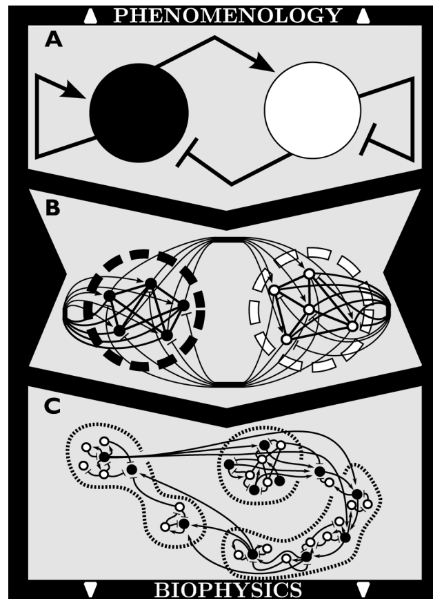
Fig 1. Multiscale top-down approach in modeling neural networks, from phenomenological to biophysical architectures. A) Neural mass model composed of excitatory (black circle) and inhibitory (white circle) populations, affected by surrounding environment (grey background). Populations act on each other via linear transfer functions, with positive gain for excitatory couplings (arrow heads) and negative gain for inhibitory couplings (flat heads). B) Single neurons (dots) are enclosed within each population (thick dashed circles). Black dots are excitatory neurons and white dots are inhibitory neurons. Linear gap junction coupling is included between neurons from the same genre (i.e. straight lines on exc—exc and inh—in connections). Non-linear synaptic coupling is introduced within and between populations (curved lines) in a fully-connected topology. C) Excitatory and inhibitory single neurons (black and white dots) are distributed spatially in a biologically relevant topological structure (thin dashed ensembles), each of which being a subset from B).
