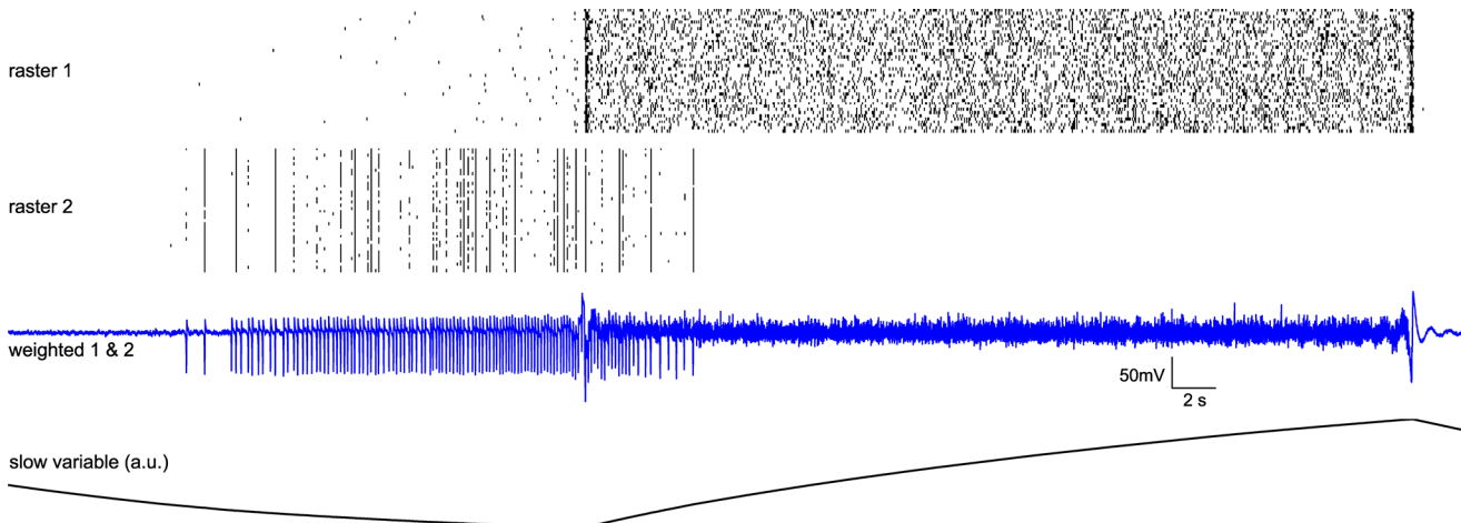
Fig 7. Simulated seizure-like event in the absence of glutamatergic and GABAergic synaptic couplings. Raster plots 1 & 2 display spikes of population 1 and 2 neurons, with activation threshold at 0 mV; third trace is the mean of the two populations with 80% contribution of excitatory ensembles and 20% contribution of inhibitory ensembles; slow permittivity variable is the z variable from Eq 3 (in arbitrary unit), mainly affected by excitatory cells, exerting an inhibitory effect on inhibitory cells upon exogenous factors; bottom plot is experimental data. Parameters: C_E = 0.8 ; x_0 = 3.0 ; W_{\max} = 0.2 ; G_s^{ij} = 0 ; G_s^{ii} = 0 ; r = 0.000004 .
