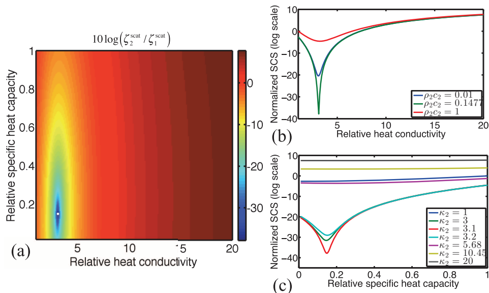
Figure 3 | Thermal scattering reduction. (a) Normalized (analytical) SCS \zeta^{\text{scat}} in logarithmic scale, versus the relative heat conductivity \kappa_2 / \kappa_0 and the relative specific heat capacity \rho_2 c_2 / \rho_0 c_0 . The white dot represents the position of optimized scattering reduction, with a value of 40 dB. The color bar denotes the plot of 10 \log(\zeta_2^{\text{scat}} / \zeta_1^{\text{scat}}) , where the subscripts 1 and 2 refer to the scattering cross-section of the obstacle and cloaked structure, respectively. (b) Normalized SCS versus the relative heat conductivity for various values of the specific heat capacity \rho_2 c_2 / \rho_0 c_0 . (c) Normalized SCS versus the relative specific heat capacity \rho_2 c_2 / \rho_0 c_0 for various values of the relative heat conductivity \kappa_2 / \kappa_0 .
