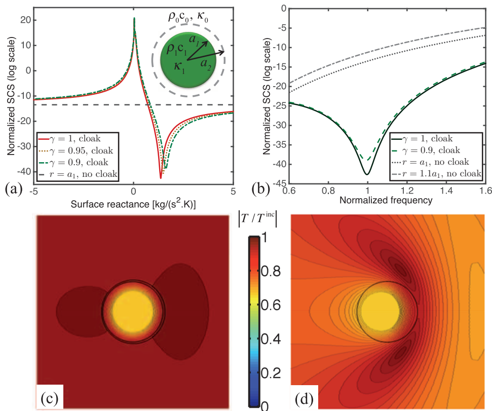
Figure 5 | Thermal mantle cloaking. Normalized (analytical) SCS \zeta^{scat} versus X_s 10^{-7} for the object with normalized radius k_0 a_1 = 0.5 and relative heat conductivity \kappa_1/\kappa_0 = 0.1 for various values of the ratio \gamma . (b) Normalized SCS \zeta^{scat} versus normalized frequency for the same object with X_s = 1.36 \times 10^{-7} and X_s = 1.62 \times 10^{-7} for values of the ratio \gamma = 1 and \gamma = 0.9 . The inset of Fig. 5(a) illustrates the object coated with a thermal metasurface, projected in the x-y plane. Amplitude of the temperature field on the x-y plane for the same object (c) with mantle cloak with X_s = 1.62 \times 10^{-7} and (d) without the cloak. The color bar denotes the plot of |T/T^{inc}| .
