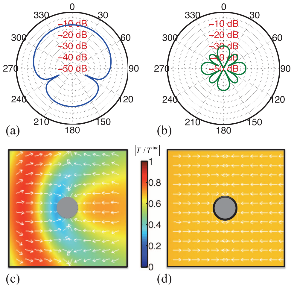
Figure 4 | Near and far-field characterization. Analytical scattering amplitude |g(\theta)| , given by Eq. (17), in polar coordinates, and in logarithmic scale (a) for the bare object with \kappa_1/\kappa_0 = 0.5 and (b) for the cloaked object, with \kappa_2/\kappa_0 = 3.1 . Amplitude of the oscillating temperature in the near-field of (c) the same bare object of Fig. 4(a) and (d) the same cloaked object of Fig. 4(b) for k_0 a_1 = 0.5 . Arrows show the direction of \nabla T and the color bar denotes the plot of |T/T^{\text{inc}}| .
