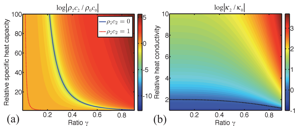
Figure 2 | Optimal cloaking parameters. (a) Relative specific heat capacity of the shell \rho_2 c_2 / \rho_0 c_0 in logarithmic scale, versus the ratio \gamma = a_1 / a_2 and the relative specific heat capacity of the object \rho_1 c_1 / \rho_0 c_0 . The color bar denotes the plot of \log|\rho_2 c_2 / \rho_0 c_0| . (b) Relative heat conductivity of the shell \kappa_2 / \kappa_0 in logarithmic scale, versus the ratio \gamma = a_1 / a_2 and the relative heat conductivity of the object \kappa_1 / \kappa_0 . The color bar denotes the plot of \log|\kappa_2 / \kappa_0| and the dashed black line represents \log|\kappa_2 / \kappa_0| = 0 .
