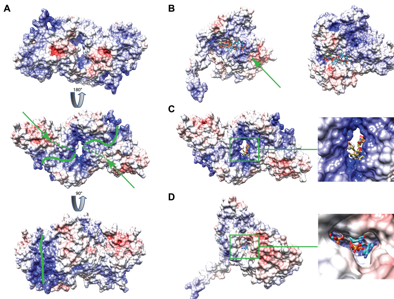
Figure 5. Electrostatic surface representation of the Mg561 protein. (A) Electrostatic surface of the Mg561 dimer. The green lines correspond to the possible RNA binding sites in the positively charged grooves (blue). The green arrows point the position of the second tunnel and the dashed lines delineate the tunnel path under the surface. Contour levels: red, V < -10 kcal/mol; white, -10 kcal/mol < V < +10 kcal/mol; blue, V > +10 kcal/mol. (B) Proposed mimivirus PAP RNA and ATP binding mode (left panel, Mg561 monomer) based on the superimposition of the VP55 complex with ATP and RNA (PDB 3ERC) on Mg561 (right panel). Predicted cation sites are marked as green balls. (C) As in (B) but with the Mg561 dimer (left panel). Close-up of the central tunnel (right panel). (D) Proposed ATP entry route pointed by the green arrow (left panel). Close-up of the tunnel through the ATP binding site (right panel).
