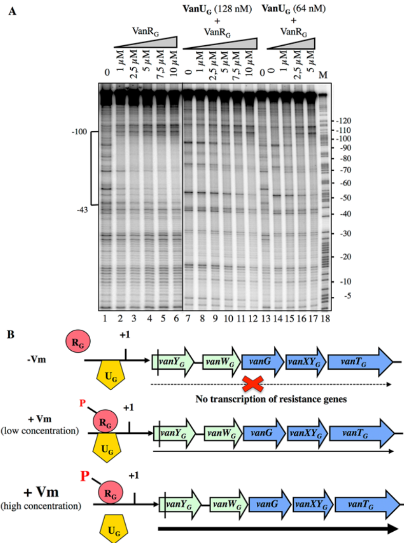
Fig 6. Competition between VanU G and VanR G for binding to the P VG resistance promoter. (A) DNase I footprinting analysis. A 233-bp DNA fragment was amplified from the P YG region using a labeled reverse primer (YG10) (S2 Table) to radiolabel the template strand. Increasing amounts of VanR G and two fixed amounts of VanU G , indicated at the top, were incubated with the DNA probe. The bracket indicates the region protected from DNase I cleavage by VanU G and/or VanR G and the co-ordinates of protection relative to the transcriptional start site are indicated on the left. M is the A+G Maxam and Gilbert sequencing reaction lane of the probes used as a size marker and the nucleotide positions are indicated at the right. (B) Model for the binding competition between VanU G and VanR G -P in the absence or in the presence of various concentrations of vancomycin (Vm).
