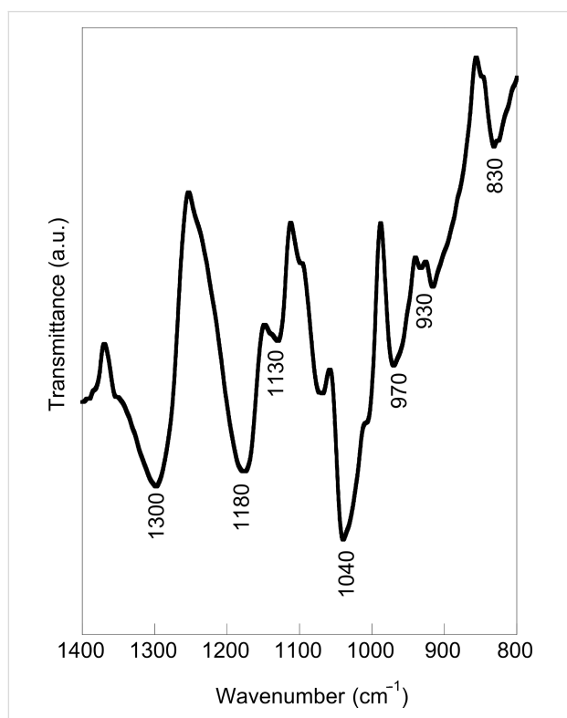
Figure 6: FTIR spectrum of a PEDOT film electropolymerized onto vitreous carbon.
