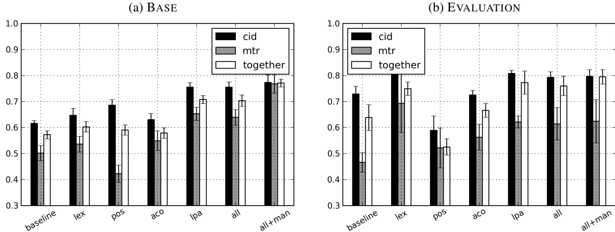
Figure 2: Classification results: f-measure (y-axis) per feature set (x-axis).
