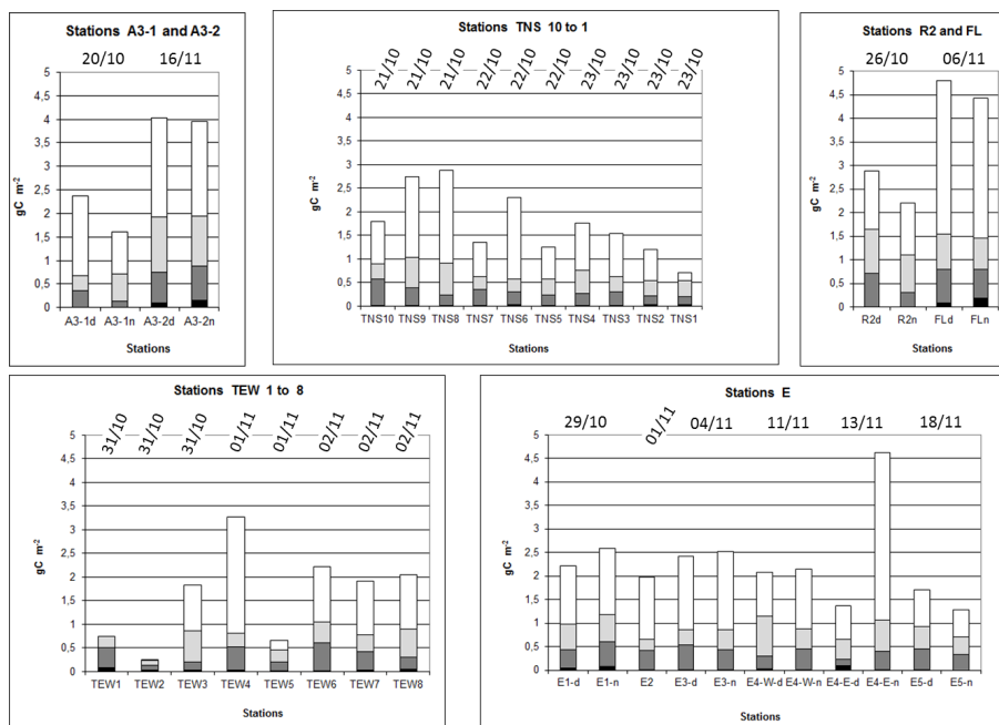
Figure 3. Integrated 0–200 m mesozooplankton biomass estimated from ZOOSCAN for the different stations sampled during KEOPS2 with size-fraction distributions. Size fractions: <500 μm, black; 500–1000 μm, dark grey; 1000–2000 μm, light grey; >2000 μm, white.
