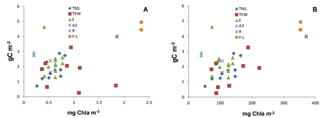
Figure 5. Zooplankton biomass values against average Chl a in the upper 100 m (a) and against the integrated Chl a in the mixed layer depth (b) for the different stations visited during KEOPS2. Biomass values from Fig. 3.
