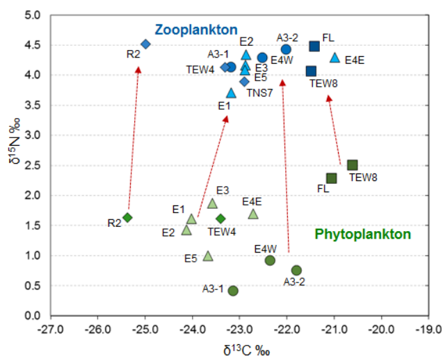
Figure 10. Mean \delta^{13}\text{C} and \delta^{15}\text{N} values of phytoplankton (5–210 \mu\text{m} ) (Trull et al., 2015) and zooplankton (200 to >2000 \mu\text{m} ) (present study) for stations sampled during the KEOPS2 cruise. Symbols correspond to the phytoplankton groups based on chemometric measurements identified by Trull et al. (2015): diamonds, T-group 1; triangles, T-group 2; dots, T-group 3; squares, T-group 5.
