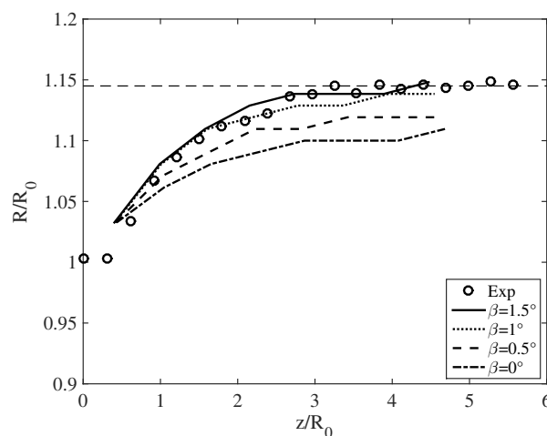
Figure 2. Downstream evolution of helix radius. \beta is the blade pitch offset.
