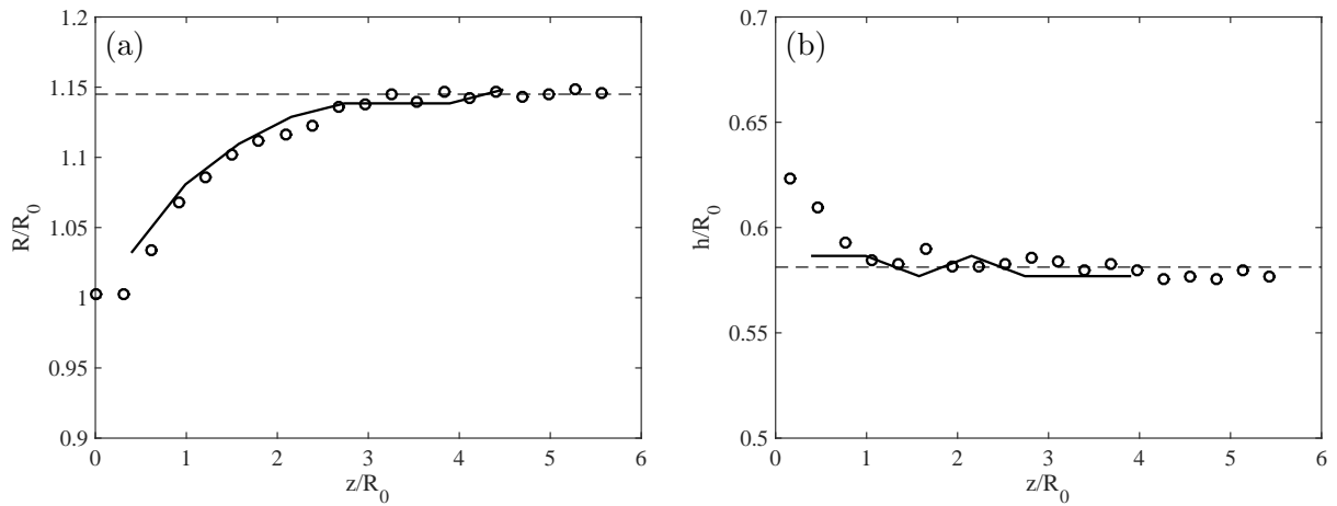
Figure 6. Downstream evolution of helix parameters: (a) radius and (b) pitch. Experiment ( \circ ) and numerical computations ( — ).
