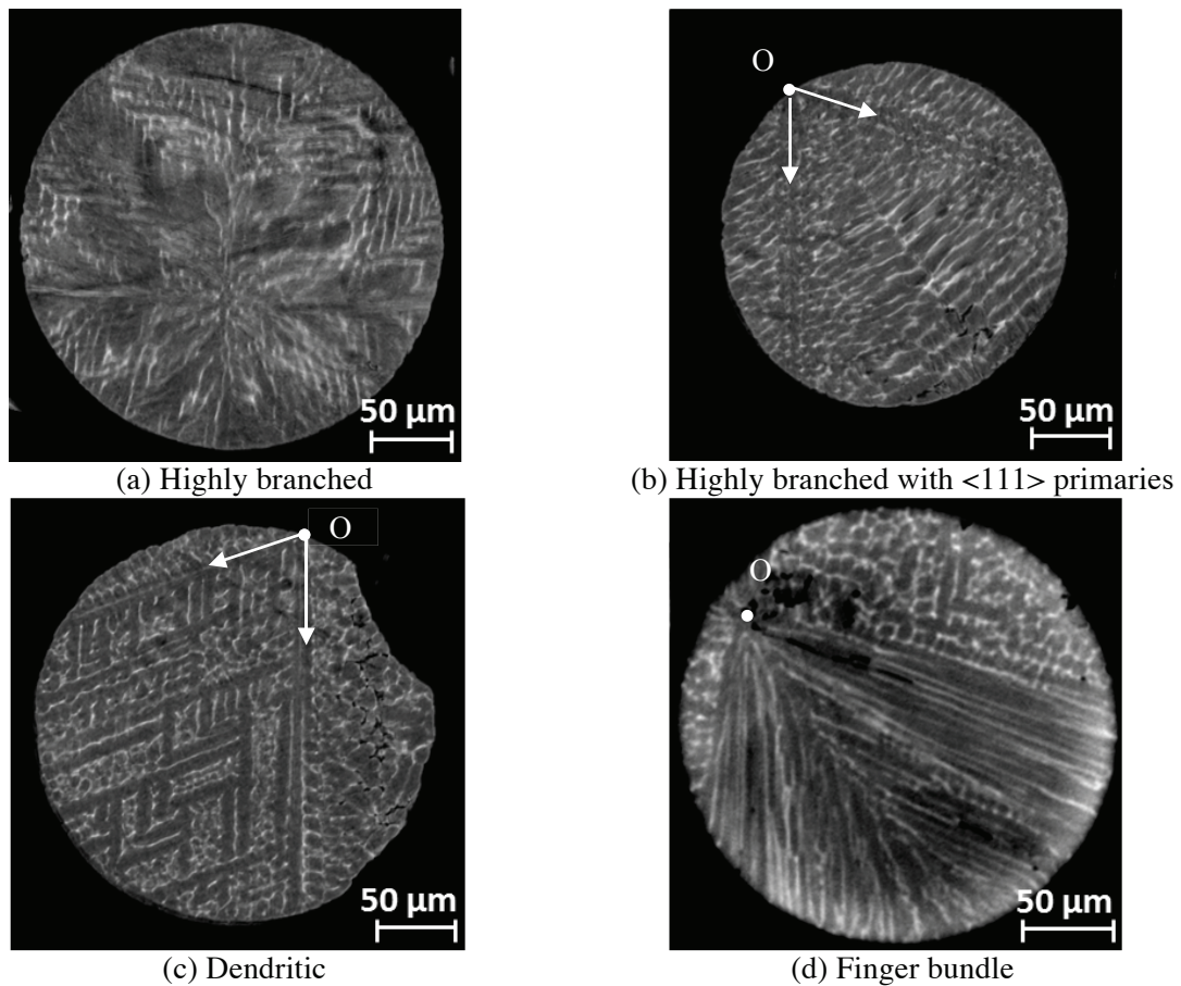
Figure 1. Examples of the four morphologies identified in the Al-4.5wt.%Cu droplets of diameter between 250 and 300 \mu\text{m} : (a) highly branched morphology, (b) highly branched morphology with visible primary arms oriented along \langle 111 \rangle directions, (c) dendritic morphology and (d) finger bundle morphology. The nucleation position noted O is shown by a white dot and the primary arms by white arrows.
