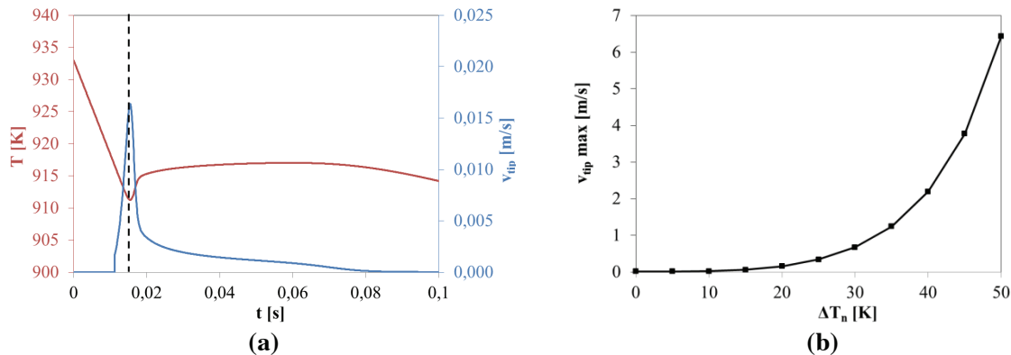
Figure 2. (a) Predicted time evolution of temperature and tip velocity during the solidification beginning of a droplet cooled in argon whose diameter is equal to 300\mu\text{m} , for a nucleation undercooling fixed at \Delta T_n = 5^\circ\text{C} . The dashed line corresponds to both the maximal tip velocity and the local minimum temperature and (b) Predicted maximal tip velocity reached during solidification of a droplet cooled in argon whose diameter is equal to 300\mu\text{m} , depending on the imposed nucleation undercooling value.
