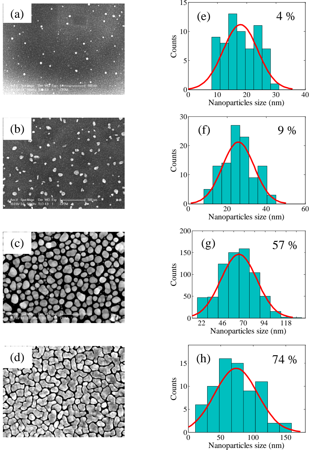
Figure 3. SEM images of Ag-NPs with mass thicknesses corresponding to (a) 5 nm, (b) 10 nm, (c) 15 nm and (d) 20 nm grown on silicon substrates and annealed at 250° C during 60 min. (e), (f), (g) and (h) correspond to the NPs size distribution, respectively.
