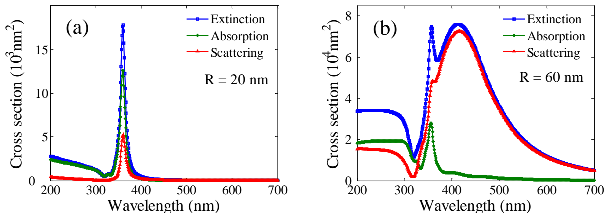
Figure 1. Calculated extinction, absorption and scattering cross sections of Ag-NPs in vacuum (air) with 20 nm (a) and 60 nm (b) radius. Measured values for the dielectric function \epsilon(\omega) are taken from Johnson and Christy database [18].
