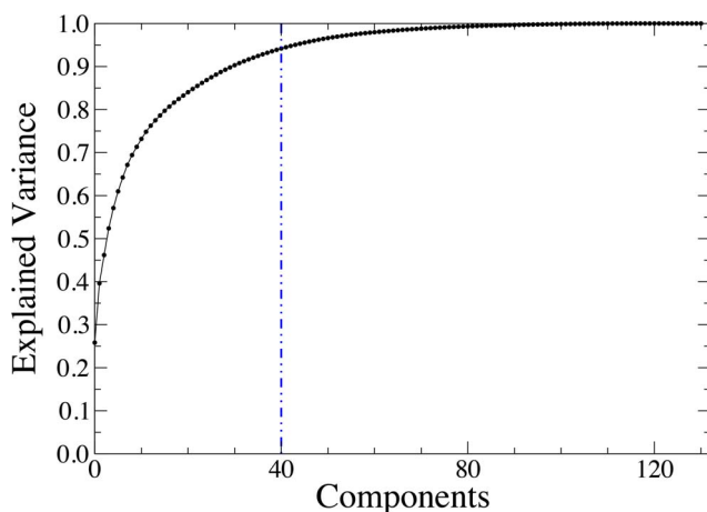
Figure 3. Cumulative variance explained as a function of the number of components. With 40 components (vertical blue line) we are able to maintain over 94% of the variance present in the data while significantly reducing the matrix size. doi:10.1371/journal.pone.0112074.g003
