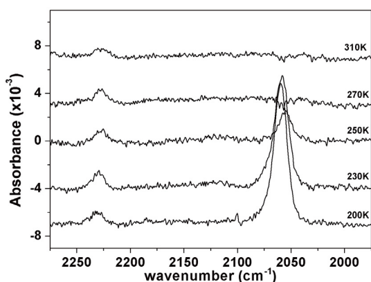
Fig. 7. Change in the range 1950\text{--}2300\text{ cm}^{-1} of the infrared spectrum after heating from 200 to 310 K and after the sublimation of methanimine, ammonia, and hydrogen cyanide (160 K). The deposit includes an excess of methanimine with respect to both \text{NH}_3 and HCN, producing traces of [\text{NH}_4^+ \text{ } ^-\text{CN}] .
