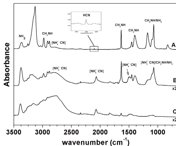
Fig. 6. Infrared spectra of methanimine/HCN/ \text{NH}_3 deposit at 20 K in the presence of either a methanimine excess (A), methanimine with a more important quantity of [\text{NH}_4^+ \text{CN}] in comparison with spectrum A (B), or an excess of [\text{NH}_4^+ \text{CN}] (C).
