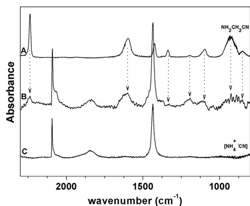
Fig. 11. Infrared spectra of aminoacetonitrile \text{NH}_2\text{CH}_2\text{CN} at 130 K (A), of refractory residue at 210 K coming from a deposit with an excess of [\text{NH}_4^+ \text{CN}^-] (B) and [\text{NH}_4^+ \text{CN}^-] salt at 160 K (C).
