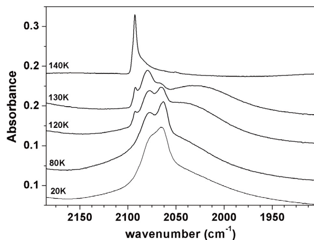
Fig. 5. Temperature evolution of the [\text{NH}_4^+ \text{CN}] salt infrared profile for the 1900–2200 \text{cm}^{-1} range.
