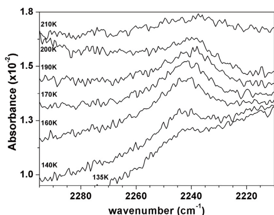
Fig. 10. Infrared spectra in the range 2215–2300 \text{cm}^{-1} relative to the thermal range 135–210 K for a deposit including an excess of [\text{NH}_4^+ \text{CN}^-] .
