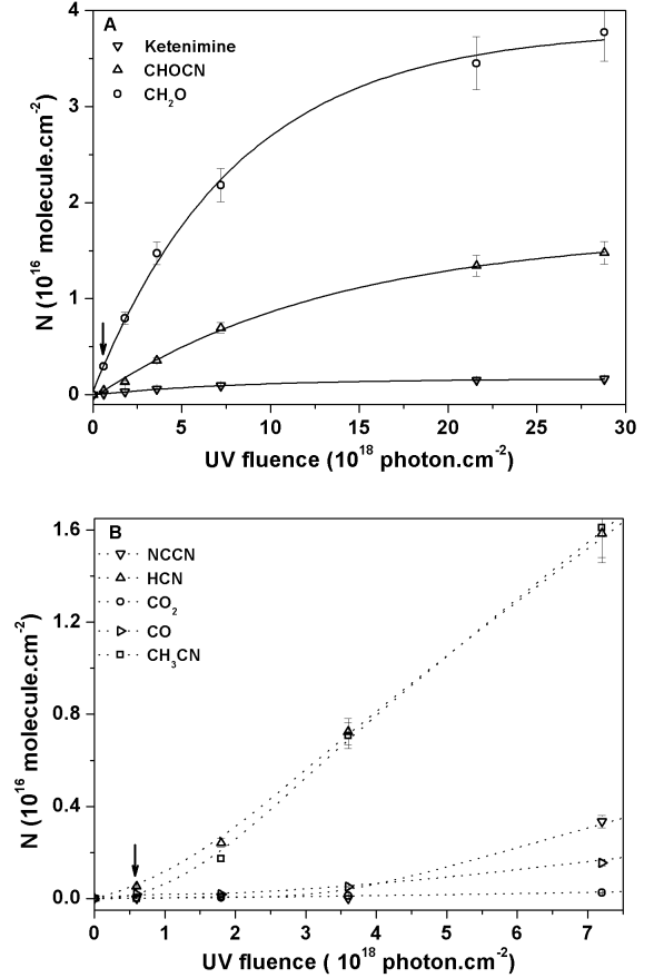
Fig. 4. Evolution of the photo-products from the primary photodegradation pathways of HOCH 2 CN at 40 K A ), and from secondary photodegradation pathways B ). The arrow refers to the time of the measurement of the photoproducts from the primary photodegradation process of HOCH 2 CN.
