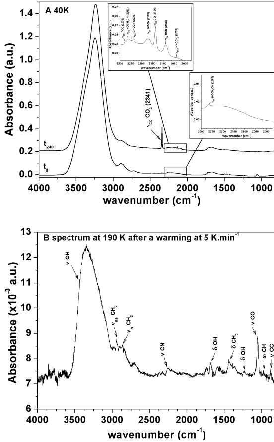
Fig. 7. UV irradiation of \text{HOCH}_2\text{CN} diluted in a water ice (1:10 \text{HOCH}_2\text{CN}:\text{H}_2\text{O} ). A) Infrared spectra monitored after the \text{H}_2\text{O}:\text{HOCH}_2\text{CN} ice formation at 40 K, t_0 , and after 240 min of VUV irradiation at 40 K, t_{240} . B) Infrared spectrum obtained at 190 K after the warming of the sample displayed in A) t_{240} with a 5 K min -1 temperature ramp. Note: vibration mode: stretching ( \nu ), bending ( \delta ), rocking ( \rho ), torsion ( \tau ), wagging ( \omega ). Type of vibration mode: asymmetric (as), symmetric (s).
