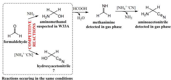
Fig. 1. Experimental pathways in astrophysical conditions for the hydroxyacetonitrile formation via the direct reaction of ammonium cyanide ( [\text{NH}_4^+ \cdot \text{CN}] pathway), and its concurrent reaction, the aminoacetonitrile formation in solid phase via the Strecker synthesis (ammonia ( \text{NH}_3 ) pathway).
