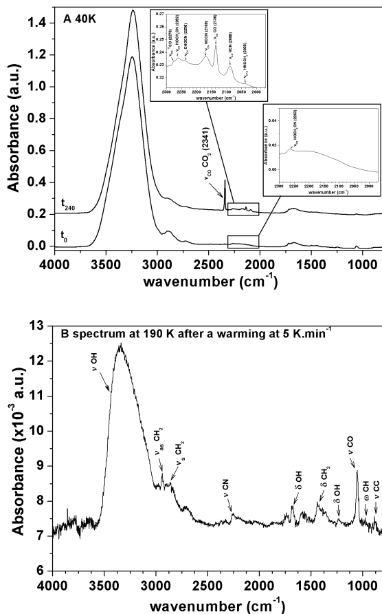
Fig. 7. UV irradiation of HOCH_2CN diluted in a water ice (1:10 HOCH_2CN:H_2O ). A ) Infrared spectra monitored after the H_2O:HOCH_2CN ice formation at 40 K, t_0 , and after 240 min of VUV irradiation at 40 K, t_{240} . B ) Infrared spectrum obtained at 190 K after the warming of the sample displayed in A ) t_{240} with a 5\text{ K min}^{-1} temperature ramp. Note: vibration mode: stretching ( \nu ), bending ( \delta ), rocking ( \rho ), torsion ( \tau ), wagging ( \omega ). Type of vibration mode: asymmetric (as), symmetric (s).
