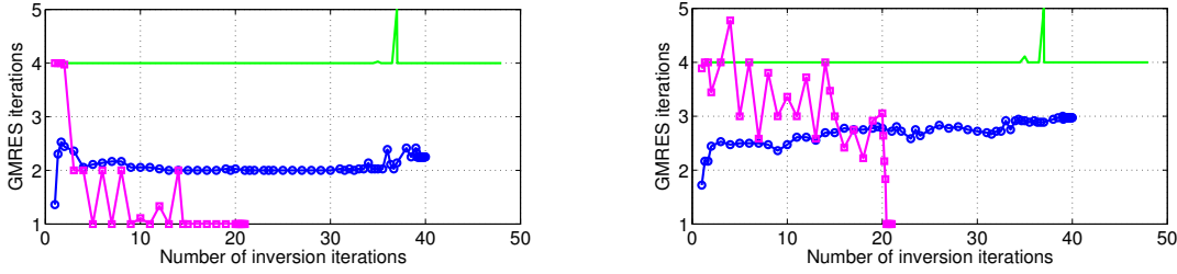
Figure 5. Average number versus the number of iterations of the inversion algorithm of the GMRES iterations obtained either with the blank initialisation (—), the marching-on-in-permittivity permittivity initialisation ( \square ), or the marching-on-in-source source initialisation ( \circ ). (Left) G values for the direct field computation and (Right) H values for the adjoint field computation.
