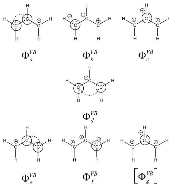
Scheme 2: VB structures for the allyl cation; the brackets around \Phi_g^{VB} indicated that this structure is removed ( \Phi_c^{VB} = \Phi_g^{VB} ). Circles represent atom-centered p orbitals.
