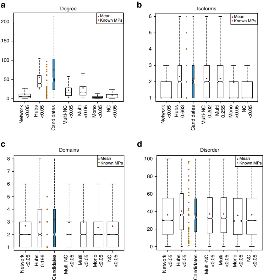
Figure 2 | Protein features. (a) Protein degree. (b) Protein isoforms. (c) The number of Pfam domains (including PfamB) predicted on each protein. (d) Protein disorder as calculated by disordered. The numbers shown are the percentage of a protein's residues that are disordered. Outliers are not shown. Red dots indicate mean values and the camel dots between Candidates and Hubs are the values of the known moonlighting proteins.
