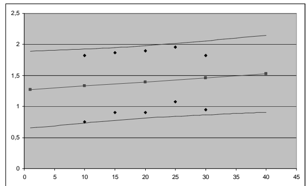
Fig.4. Statistical limit of the matter
