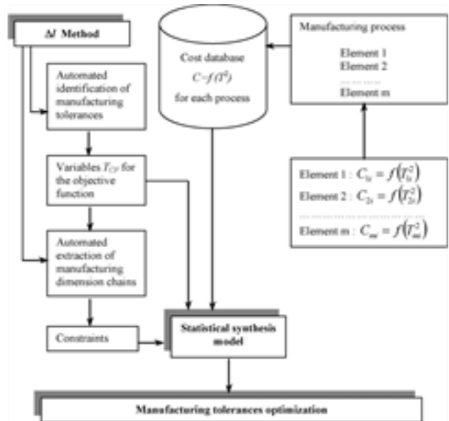
Figure 7. Flowchart of the optimization procedure.
