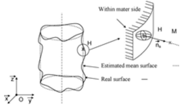
Fig. 11. Variance of point H.
