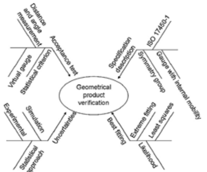
Fig. 2. Fields of geometrical verification with a CMM.
