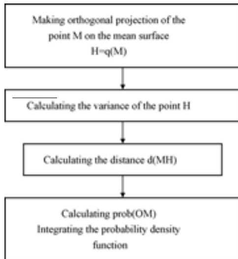
Fig. 10. The steps in calculating prob(M).
