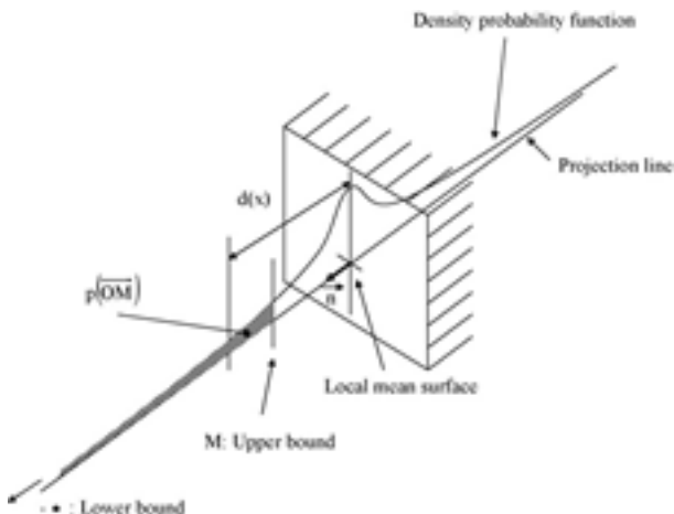
Fig. 13. Integrating the probability density function.
