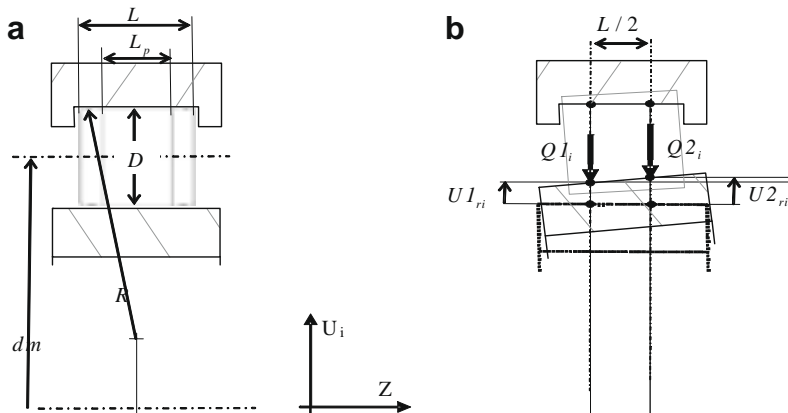
Fig. 9. (a) Roller bearing geometry; and (b) relative displacements in the section of roller i .
