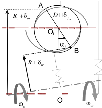
Fig. 10. Kinematic model of ball bearing under load.
