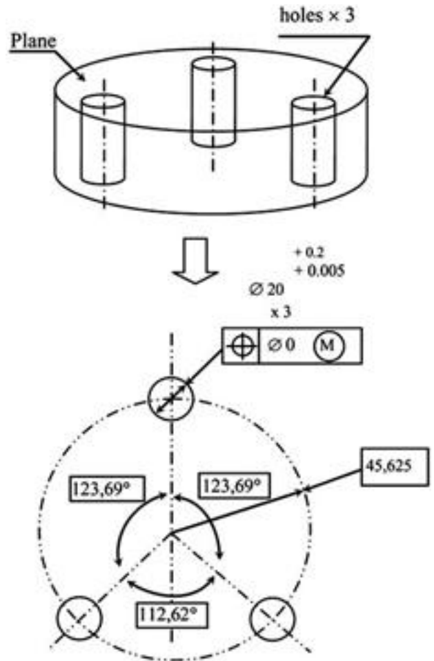
Fig. (3). Tolerancing suggested.
