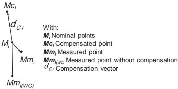
Fig. 12. Employed notations.
