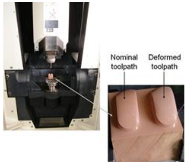
Fig. 11 Experimental part
