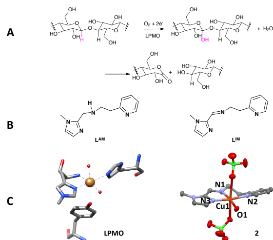
Figure 1. A) Oxidative cleavage of polysaccharides catalyzed by LPMO. B) Ligands used in the present study. C) Active site of LPMO from Thermoascus aurantiacus (pdb 2yet) and ORTEP diagram of complex 2 (30% thermal ellipsoid plots). Hydrogen atoms were omitted for clarity. Selected distances in Å: Cu1-N1: 2.000(2), Cu1-N2: 2.001(2), Cu1-N3: 1.973(2), Cu1-O1: 1.9771(19).
