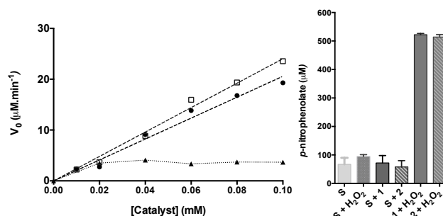
Figure 2. Reaction of p -nitrophenyl- \beta -D-glucopyranoside (S) with complexes 1 and 2 and H 2 O 2 in carbonate buffer 100 mM pH 10.5 and at 30°C with [H 2 O 2 ]=20 mM and [S] =20 mM. Left: initial velocities as a function of complex concentration for complexes 1 (●) and 2 (□) and for CuSO 4 (▲) Right: concentration of p -nitrophenolate obtained after 24 hours of reaction with [ 1 or 2 ]=0.01 mM.
