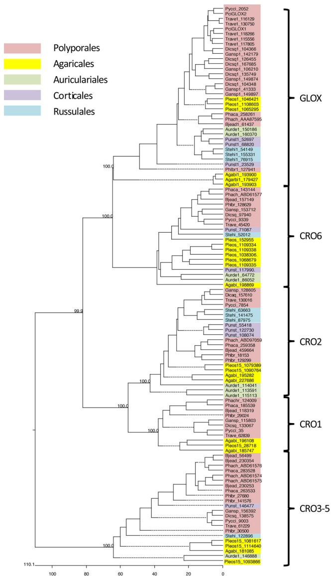
FIG 1 Phylogenetic tree showing relationships among predicted CRO proteins derived from representative white rot fungi, including P. cinnabarinus and P. chrysosporium . ClustalW alignments and tree construction followed the manual deletion of secretion signals and, in the case of CRO3 to CRO5, the removal of repetitive N-terminal WSC domains. On the basis of 1,000 trials, bootstrap values are shown at key nodes. Substitutions were calculated by use of the Kimura distance formula. Taxonomic orders are highlighted by colored shading. Trave, Trametes versicolor ; Dicsq, Dichomitus squalens ; Gansp, a Ganoderma sp.; Phaca, Phanerochaete carnosae ; Bjead, Bjerkandera adusta ; Phlbr, Phlebia brevispora ; Pci and Pycci, Pycnoporus cinnabarinus ; Pleos, Pleurotus ostreatus ; Agabi, Agaricus bisporus ; Aurde, Auricularia delicata ; Punst, Punctularia strigozonata ; Stehi, Stereum hirsutum .
