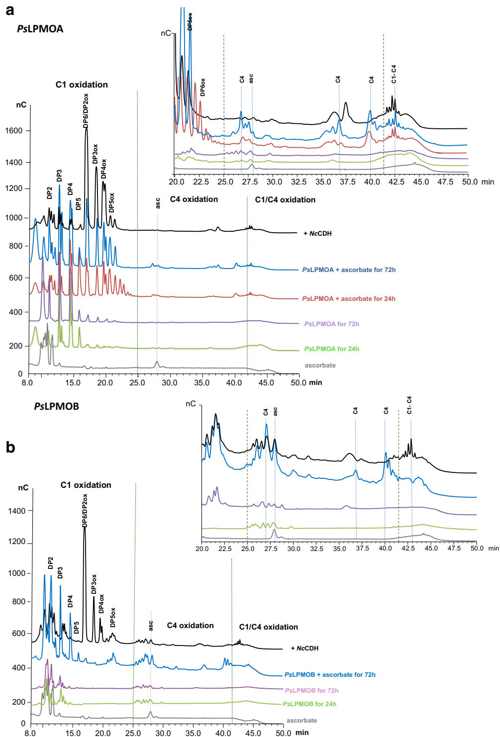
Fig. 4 Analysis of oxidized products generated from cellulose by action of PsLPMOA . a HPAEC chromatograms of the oligosaccharides products released by action of PsLPMOA . b HPAEC chromatograms of the oligosaccharides products released by action of PsLPMOB . The peak annotations are based on comparison with oligosaccharide standards oxidized at the C1 position (DP2ox-DP5ox). Peaks eluting at 27, 37, and 41 min are annotated with dotted lines. Controls ascorbate (gray line), PsLPMO with PASC for 24 h (green line) or 72 h (purple line). Reaction samples PASC (0.1 %) with 4.4 \mu M PsLPMOs in the presence of 1 mM ascorbate, at 50 ^{\circ} C for 24 h (blue line) or 72 h (red line), and same reaction followed by the incubation with NcCDH at 50 ^{\circ} C for 16 h (black line)
