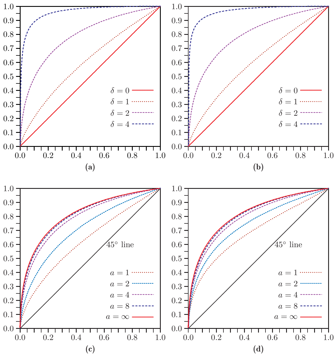
Figure 13. Size-power curves for q = 2, n = 400, \rho = 0.5, and \theta = 0 . (a) LR': a = 4 and several values of \delta ; (b) S' : a = 4 and several values of \delta ; (c) LR': \delta = 2 and several values of a ; (d) S' : \delta = 2 and several values of a .
