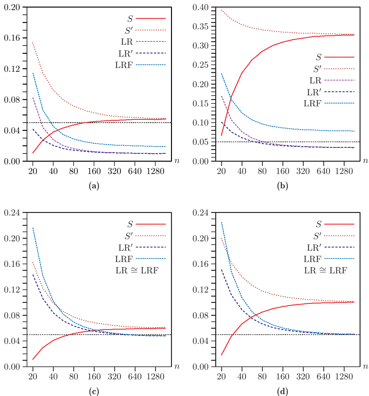
Figure 1. Rejection frequencies for asymptotic tests as functions of n for q = 8 . (a) a = 2 , \rho = 0.5 ; (b) a = 2 , \rho = 0.9 ; (c) a = 8 , \rho = 0.5 ; (d) a = 8 , \rho = 0.9 . Note that the scale of the vertical axis differs across panels.
