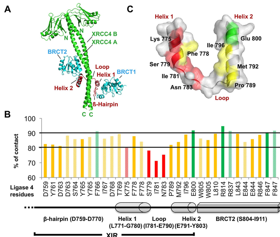
Figure 1. Structure of the human XRCC4/Lig4 complex and analysis of persistent contacts by Molecular Dynamics Simulation. (A) Crystal structure of the XRCC4/C-ter Lig4 complex (PDB entry 3II6) : the clamp domain (helix1-loop-helix2) is in red. (B) Distribution within the Lig4 C-ter domain of persistent contacts with XRCC4. Dashed and full boxes correspond to residues contacting XRCC4 A and B chains, respectively. Green, yellow and red colors highlight very persistent (contact > 90%), persistent (80% < contact < 90%) and poorly persistent (contact < 80%) residues, respectively. (C) Cartoon and surface representation of residues within the Lig4 clamp domain according to persistent contacts with XRCC4. The colors correspond to residues as in B.
