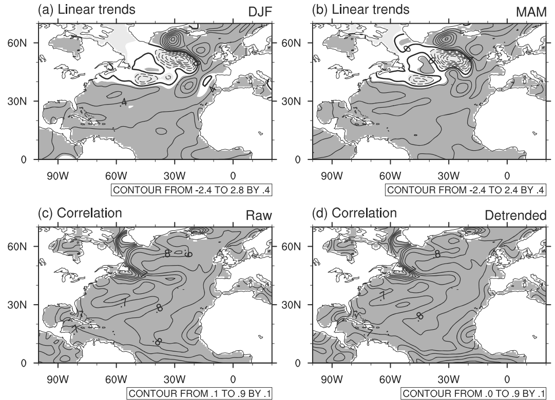
Figure 2. Changing trends ( ^{\circ}\text{C}/9.5\text{ ka} ) in (a) winter and (b) spring North Atlantic SSTs during the Holocene as estimated in the KCM HT simulation. Point-to-point correlations between December–February (DJF) and March–May (MAM) SSTs on interannual to interdecadal timescales (c) without and (d) with the removal of linear trends (insolation forcing). Dark (light) shading indicates areas where trends (correlations) are positively (negatively) significant at the 99% confidence level.
