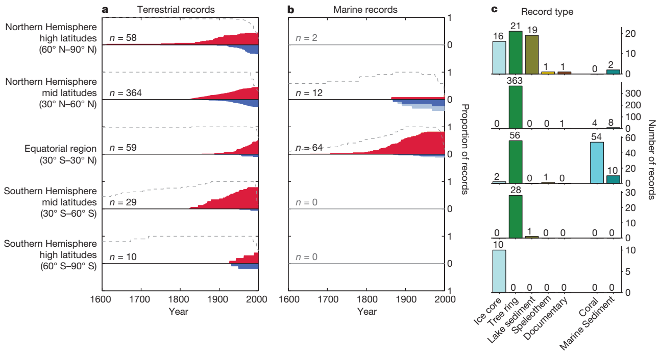
Figure 4 | Latitudinal development of site-level temperature trends. a, b, Cumulative distributions for terrestrial ( a ) and marine ( b ) records, showing latitudinal development of sustained significant warming (red; upward) or cooling (blue; downward) trends across the site-level records (Extended Data Fig. 6). The distributions are expressed as a proportion of total records within each latitudinal band (number of total records, n , indicated; grey values indicate an insufficient number of site-level records ( n \leq 2 ) for meaningful comparison). Light shading in b denotes trends at marine sediment core sites with an a priori upwelling regime (Extended
