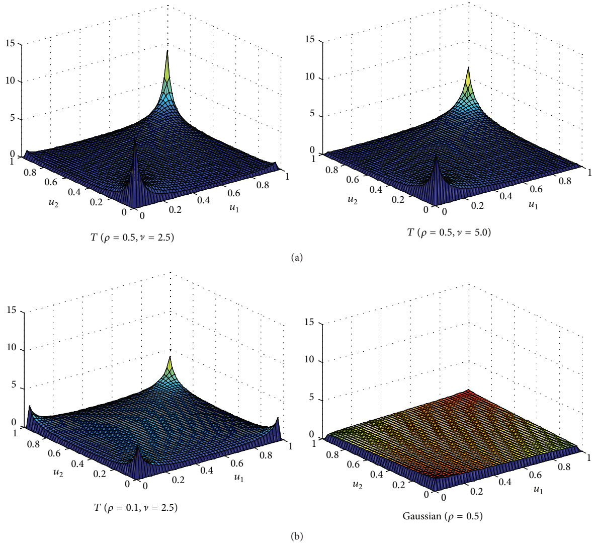
FIGURE 1: Four detailed pictures of Copula density functions. To visualize their joint probability distributions and dependence structures between variables, this figure shows the surface of the densities for Gaussian and Student’s T Copulas with various parameter values. The formulas of two Copula densities can be referred to Cherubini et al. [17]. Gaussian Copula only has one parameter, the correlation coefficient \rho . While Student’s T Copula has two parameters, the correlation coefficient \rho and the degree of freedom \nu , the latter controls the level dependence in tails. And when \nu approaches infinity, the Student’s T Copula would degenerate to Gaussian Copula.
