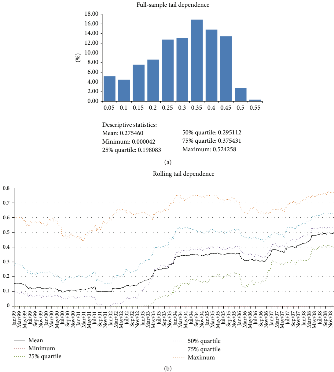
FIGURE 2: The existence of tail dependence. To verify the existence of tail dependence, we show the distribution of full-sample (1997–2008) tail dependence by the histogram and the related statistics in (a). At each time t , we employ previous two years’ observations to estimate the tail dependences for all stocks and provide the dynamics of their mean, minimum, three quartiles, and maximum from 1999 to 2008 in (b).
