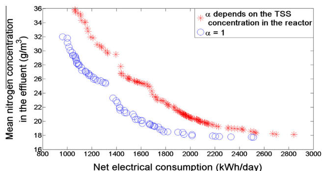
Fig. 4. Effect of the reduction of the oxygen transfer rate on the Pareto front [47].
