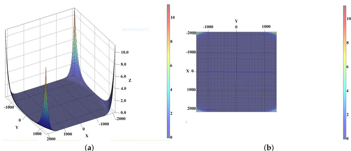
Figure 5. Inverse residual distortion with k_1 \dots k_9 coef. Computed on the entire frame. (a) Axonometric view; (b) Top view.
