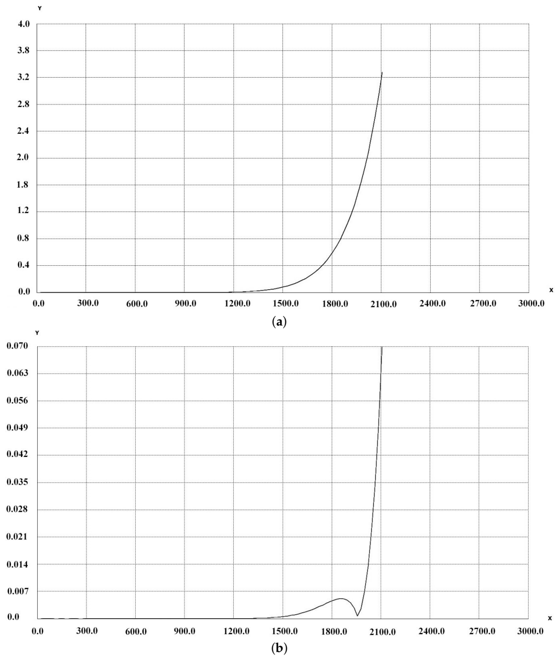
Figure 4. Inverse residual distortion with k_1..k_9 Coefficient Computed for the entire frame. (a) Inverse residual distortion with k_1..k_4 Coefficient Computed from 0 to max X frame; (b) Inverse residual distortion with k_1..k_9 Coefficient Computed from 0 to max X frame.
