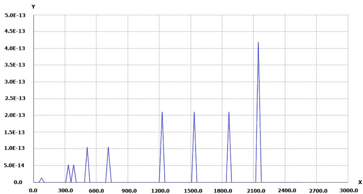
Figure 3. Iterative method applied to a Nikon D700 camera with a 14mm lens. Along the frame diagonal the points are first compensated by what is a normal process of the radial distortion using Equation (1) and then the distortion is applied with the iterative process [40] and the result compared to the original point. On Y-axis, the distance between the original point and the computed reverse point.
