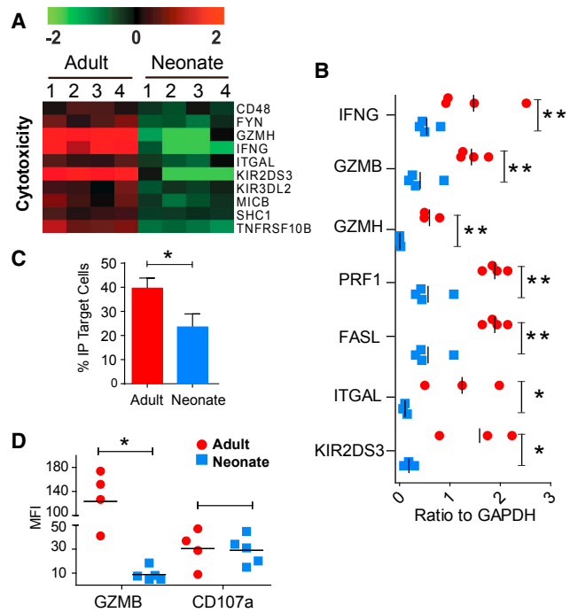
Figure 3. Adult CD8 + T Cells Are Enriched in Cytotoxicity-Related Genes
