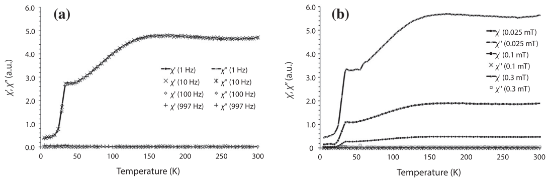
Fig. 8. 'In-phase' \chi' and 'out-of-phase' \chi'' components of magnetic susceptibility \chi_0 of 'mpo1' versus temperature in the 5–300 K temperature range at different frequencies F and field amplitudes B . (a) F_1 = 1 Hz, F_2 = 10 Hz, F_3 = 100 Hz, F_4 = 997 Hz; B = 0.025 mT; (b) F = 1 Hz, B_1 = 0.025 mT, B_2 = 0.1 mT and B_3 = 0.3 mT. "a.u." is for arbitrary units.
