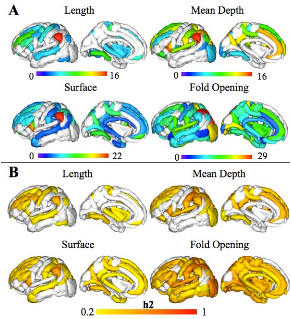
Figure 4: Heritability of bilaterally averaged sulcal measures (univariate analysis). (a) p -value (corrected for multiple tests) mapped on left hemisphere sulcal models [12]; (b) Heritability ( h^2 ) for the 4 descriptors.
