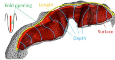
Figure 1: The four shape descriptors (fold opening, length, mean depth, and total surface area) analyzed for each sulcus.
