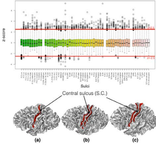
Figure 2: Top: boxplots for the z-scores across subjects. The sulci with |z|>2.5 were discarded from further analyze. Bottom: (a) a subject with a well-defined central sulcus (S.C.) and (b-c) two subjects whose S.C. was mislabeled.
