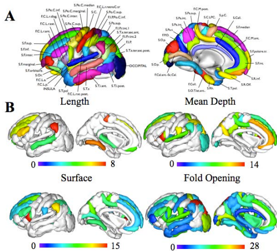
Figure 3: A) BrainVISA sulcal model B) Sulcal-based genetic correlations between left and right hemispheres (bivariate analysis). The -\log_{10} of the p -value (corrected for multiple tests) per sulcus is mapped on the left hemisphere sulcal model used for automatic labeling [12].
