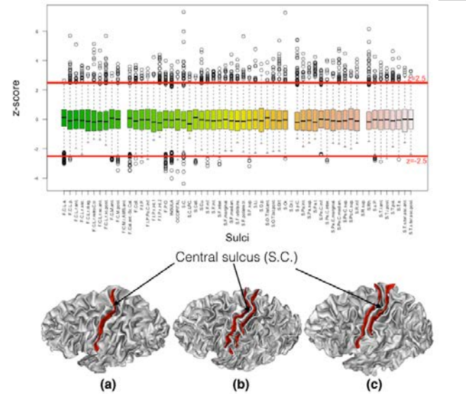
Figure 2: Top: boxplots for the z-scores across subjects. The sulci with |z|>2.5 were discarded from further analyze. Bottom: (a) a subject with a well-defined central sulcus (S.C.) and (b-c) two subjects whose S.C. was mislabeled.
