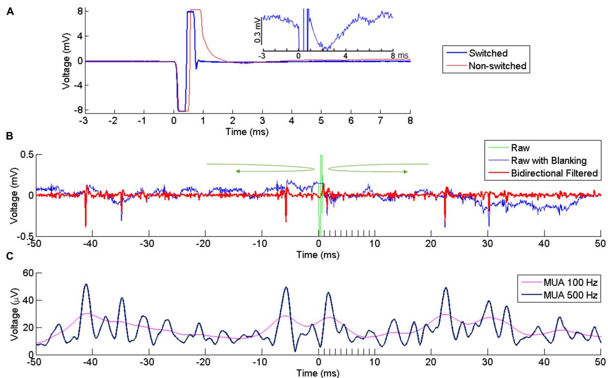
FIGURE 2 | Artifact reduction and extraction of neural signal. (A) Artifact at a recording channel 400 \mu m away from the stimulating channel with (blue) our without (red) switching between stimulating and recording modes. Time 0 indicates the onset of stimulation. The stimulation lasts for \sim 0.5 ms, resulting in the first negative phase of the artifact. In the non-switched mode, the artifact lasts for more than 0.5 ms after the offset of stimulation due to saturation of the amplifier. The long tail of the artifact is suppressed in the switched-mode, allowing fast recovery of neural activity after the stimulation offset. The inset plot shows the response in the switched mode at higher amplitude resolution. (B) Superimposed broadband signal with the stimulation artifact (green), broadband signal after artifact replacement (blue) and its high-pass filtered version (red) following bidirectional filtering separately applied to the pre-stimulus and post-stimulus signal, in the direction indicated by the green arrows. A clear spike is visible right after stimulus offset. (C) MUA computed from the signal in (B) , using two different cutoff frequencies (100 and 500 Hz).
