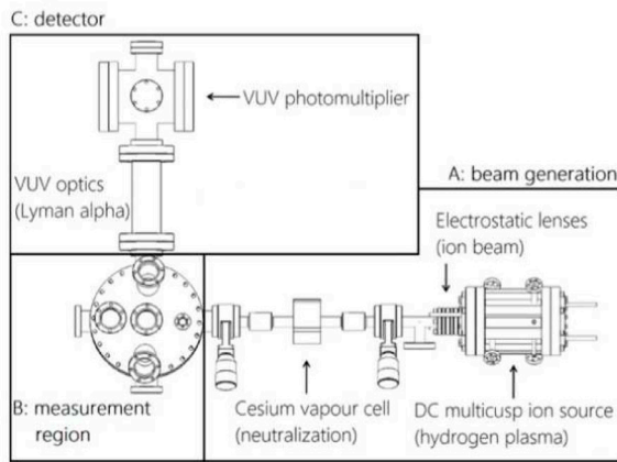
Figure 3. Scheme and photo of the experimental setup.
