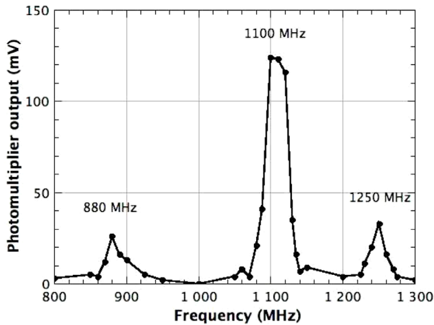
Figure 7. Photomultiplier signal as a function of the electric field frequency.
