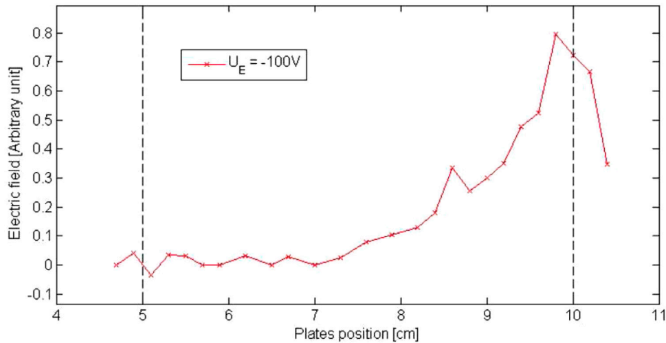
Figure 5. Electric field profile in a plasma.
