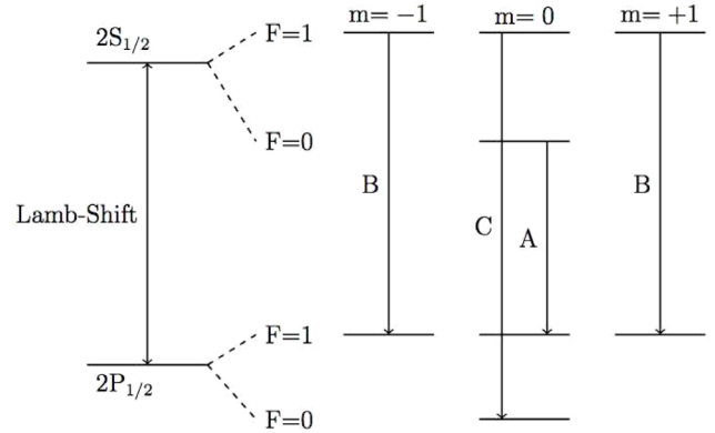
Figure 1. Hyperfine states and transitions: A = 909.67 MHz, B = 1087.4 MHz, C = 1146.6 MHz.
