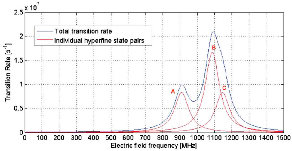
Figure 2. Total transition rate.
