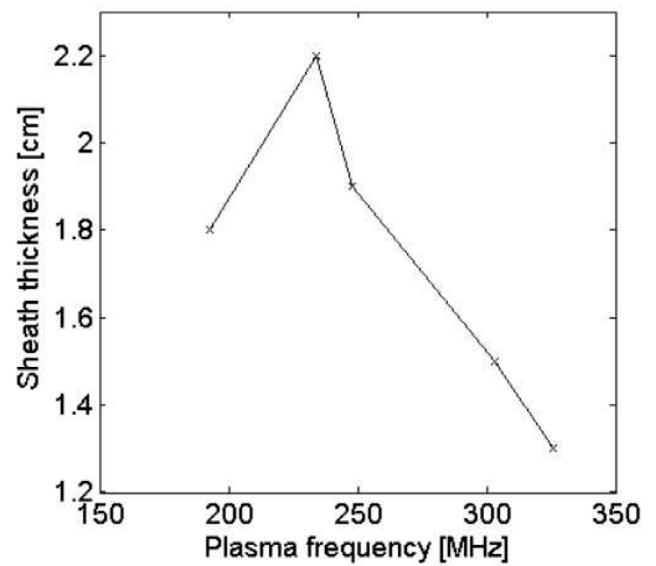
Figure 6. Sheath thickness versus plasma frequency I_d = 0.95 \pm 0.01 A, U_d = 80 V, p = (1.8 \pm 0.2) \cdot 10^{-5} mbar, I'_d = 0.13\text{--}0.65 \pm 0.05 A, U'_d = 100 V, p' = (1.1 \pm 0.1) \cdot 10^{-3} mbar.
