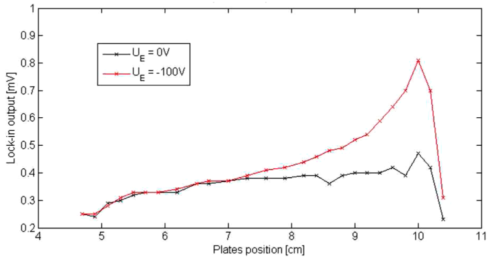
Figure 4. Electric field profile in a plasma: raw data I_d = 0.95 \pm 0.01 A, U_d = 80 V, p = (1.8 \pm 0.2) \cdot 10^{-5} mbar, I'_d = 0.26 \pm 0.05 A, U'_d = 50 V, p' = (5.1 \pm 0.2) \cdot 10^{-4} mbar.
