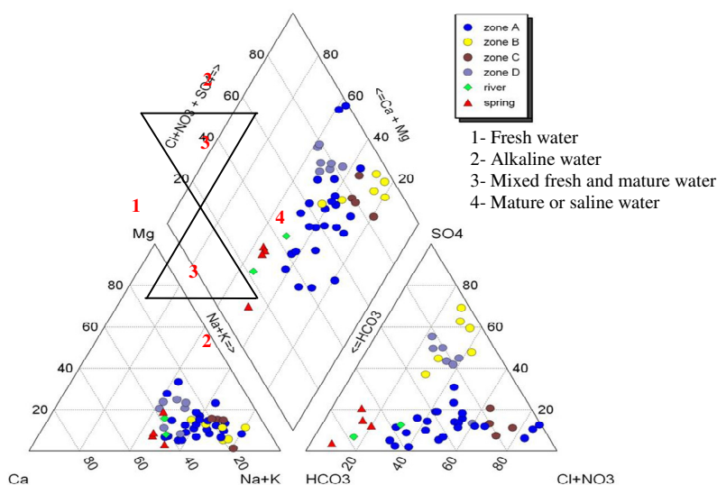
Figure-4 Piper diagram for all samples
