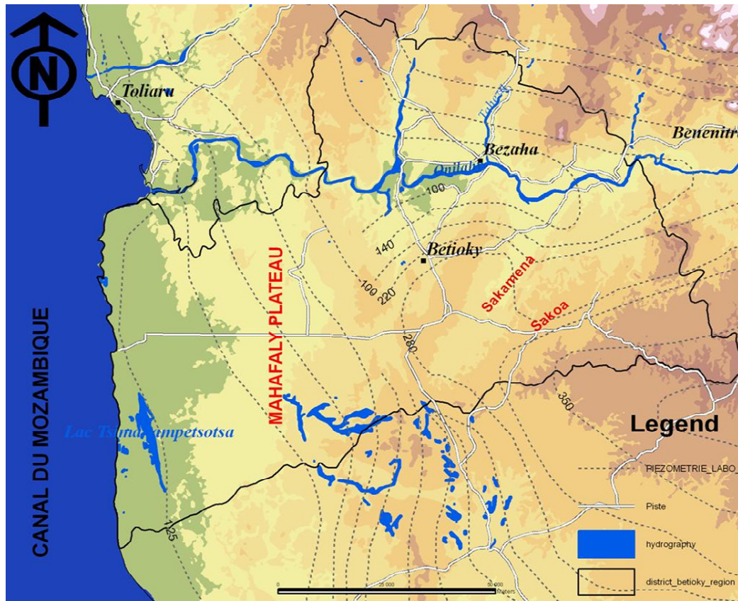
Figure-3 Piezometric map of the study area
