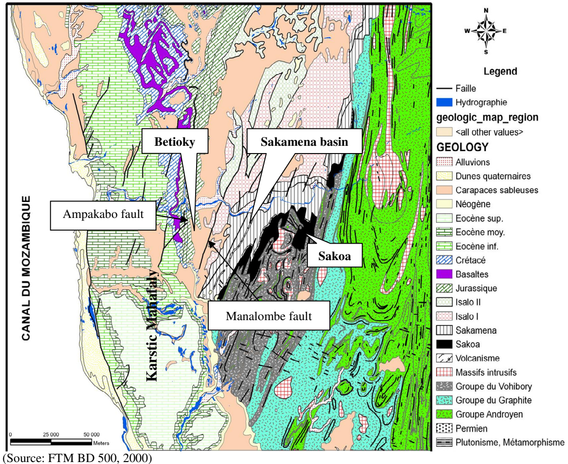
Figure-2 Geological map of study zone
