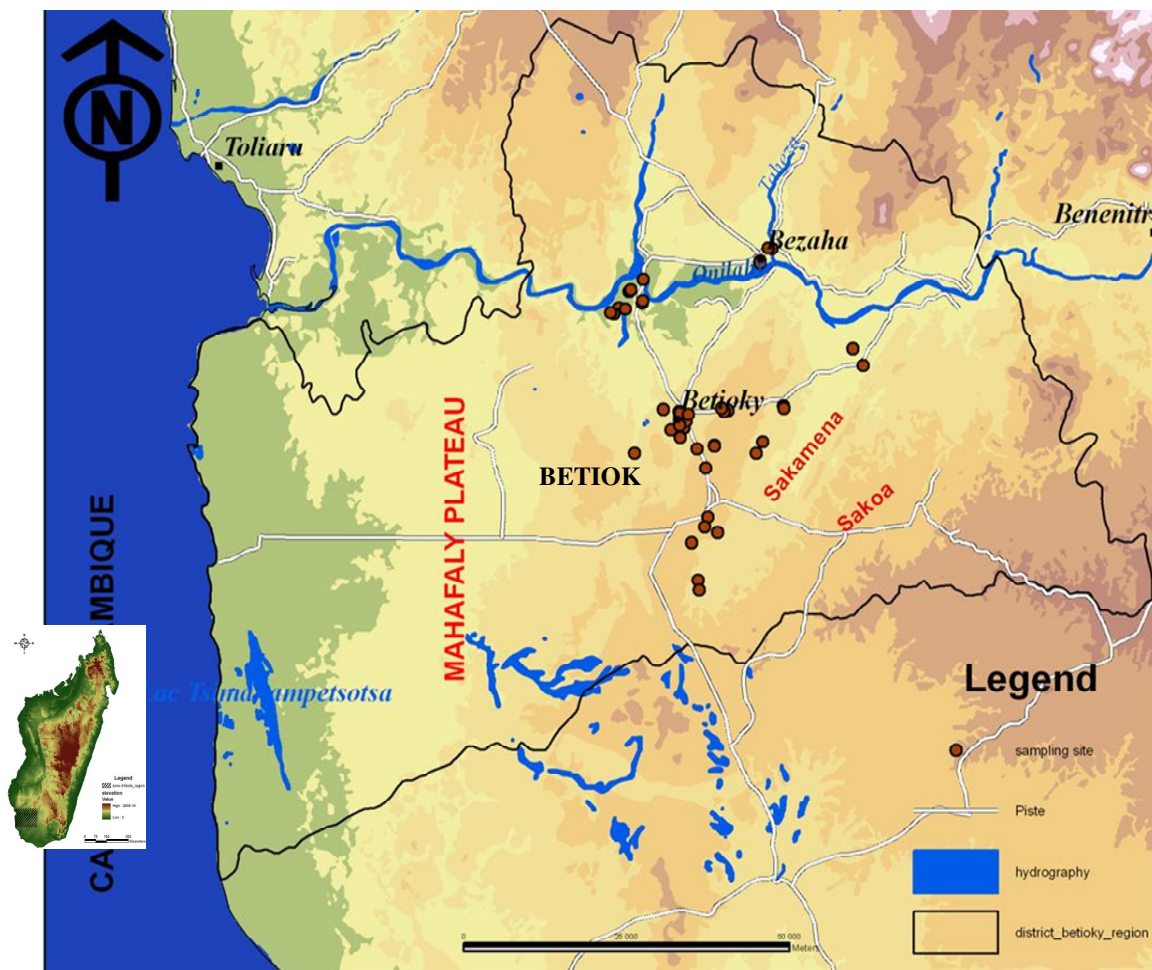
(Source: FTM BD 500, 2000)
