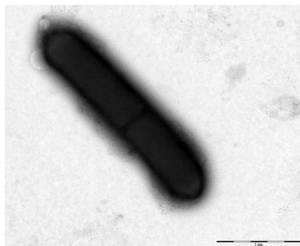
FIG. 5. Transmission electron microscopy of Massilioclostridium coli strain Marseille-P2976 T using Morgani 268D (Philips, Amsterdam, The Netherlands) at operating voltage of 60 kV. Scale bar = 1 μm.
