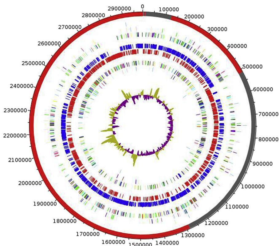
FIG. 6. Graphical circular map of chromosome. From outside to center: genes on forward strain coloured by COGs categories (only gene assigned to COGs), RNA genes (tRNAs green, rRNAs red), GC content and GC skew. COGs, Clusters of Orthologous Groups database.
