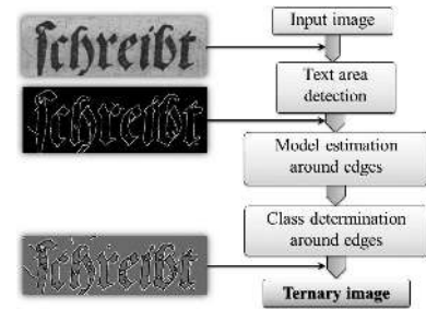
Fig. 3. Details on the sub-process S-FAIR.
