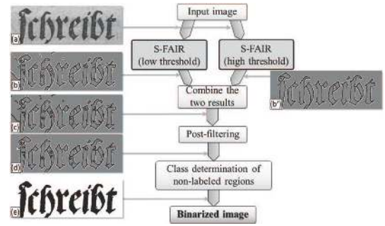
Fig. 2. Block diagram of the proposed algorithm (see section II-B for a complete description).
