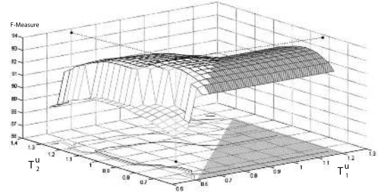
Fig. 9. Evolution of the F-Measures as function of T_u^1 and T_u^2 (means calculated on 54 images). The shaded area corresponds to parameter combinations that avoid the use of double thresholding ( T_u^1 > T_u^2 ).
