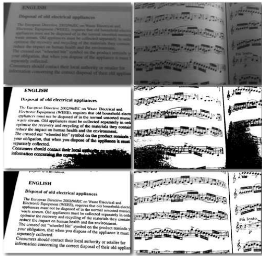
Fig. 10. Binarization of live images using a smartphone. (top) Grey input, (middle) Otsu's method, (bottom) proposed method.
