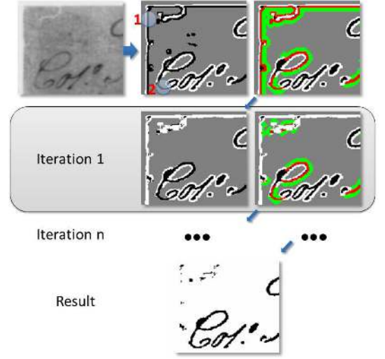
Fig. 6. Detection of misclassified text pixels. First row: (left) Input image, (middle) Three-values image created by the fusion stage, (right) in red, the problematic text pixels ( Zp_t^i ) and in green, the surrounding area used to compute labels ( Zp_b^i ). Second row: a new ternary image is produced using N_f(s) and the process reiterate until convergence.
