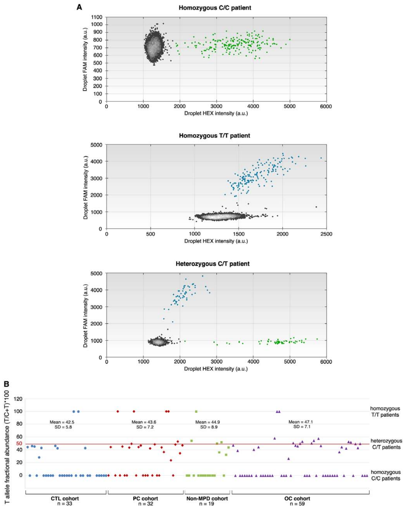
Figure 2: ddPCR analyses. The HEX-labeled probe recognizing C target SNP is visualized on the X axis and the 6-FAM labeled probe recognizing T target SNP is visualized on the Y axis. Data from three patients: A. Homozygous C patient (upper panel), homozygous T patient (middle panel) and heterozygous C/T patient (lower panel), and B. T fractional abundance [(T/(C+T)) \cdot 100] for individuals in examined cohorts.
