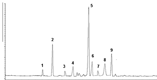
Figure 3 GC-FID chromatogram of sterols from E. elaterium seed oil. 1: Desmosterol, 2: Campesterol, 3: Stigmasterol, 4: Delta-7-Campesterol, 5: \beta -sitosterol, 6: Sitostanol, 7: Delta-5-Avenasterol, 8: Delta-7-Stigmastenol, 9: Delta-7-Avenasterol.
