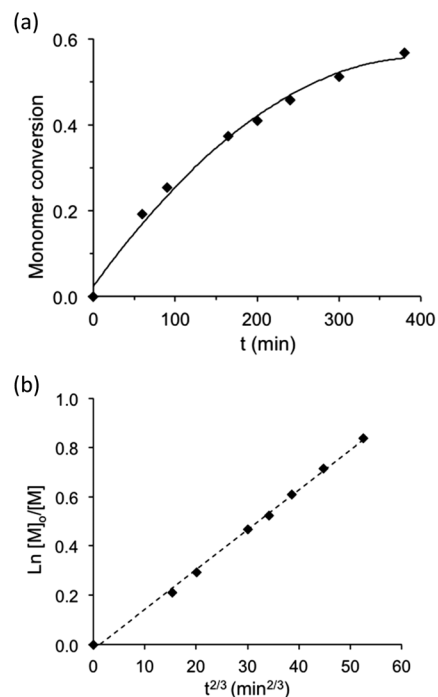
Fig. 5 Evolution of (a) monomer conversion vs. t and (b) \ln([M]_0/[M]) vs. t^{2/3} for the NMP of potassium propyl acrylate-STFSI in water solution at 100 °C using sodium MAMA-SG1 as the initiator in the presence of 7 mol% of free SG1.
