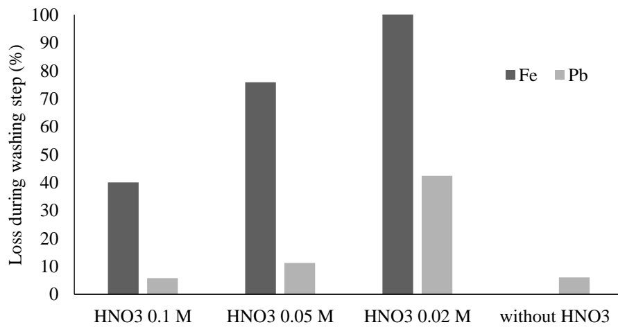
2 Fig. 3. Iron and lead washing out during washing step [multi-metal solution at 0.037 mmol.L -1 3 (V = 30 mL at 3 mL.min -1 ), nitric acid at 5 mL.min -1 (V = 9 mL for conditioning step, V = 6 4 mL for washing step), ammonium oxalate at 0.1 mol.L -1 (V = 10 mL at 4 mL.min -1 ).
