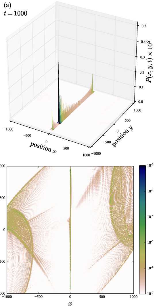
Fig. 3. Position probability of a quantum walk with an interface between two regions having distinct topology: P = |\psi_{\downarrow}|^2 + |\psi_{\uparrow}|^2 . The top panel (a) shows that the walker distribution at time t = 1000 , is essentially concentrated along the interface. The bottom panel (b) shows the same data in a logarithmic scale to reveal the structure of the small amplitudes (the wave folding due to the periodic boundary is not visible in a linear scale).
