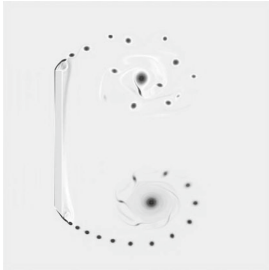
Fig. 3 Vorticity field (zoom) at t = 1.4 for the impulsively started plate at Re = 9500
